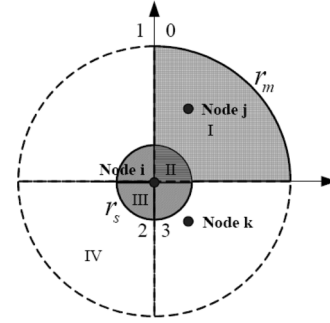
Fig. 5. The communication area of a node i in DTOR networks when directional antennas have four beam directions.
